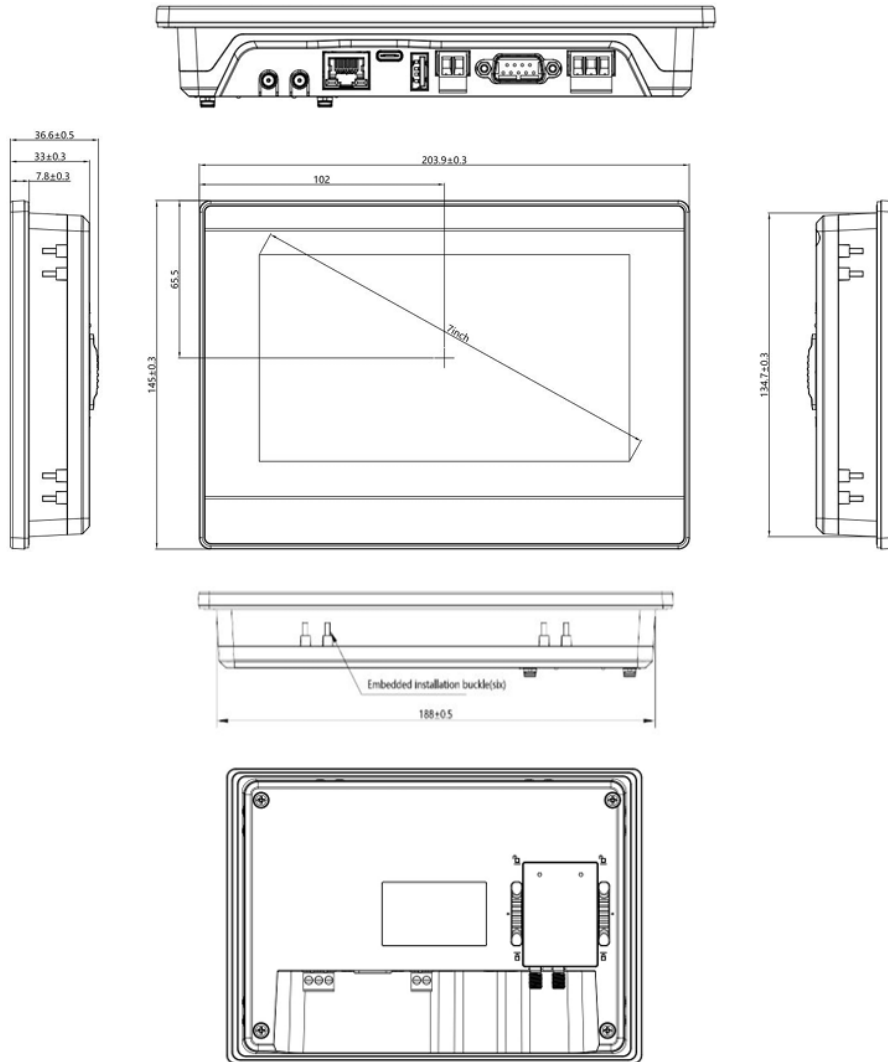
Flush-mounted installation cutout dimensions: 190 \times 136 (+1.5mm/-0.0mm)
