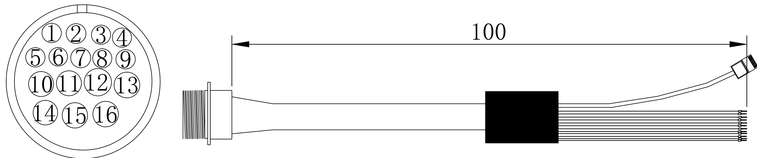
Connection Diagram
