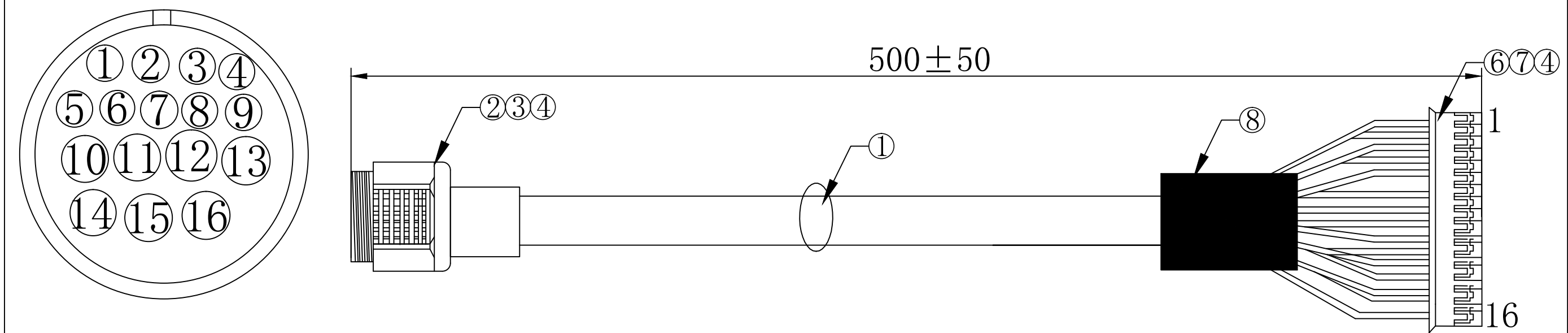
Connection Diagram
